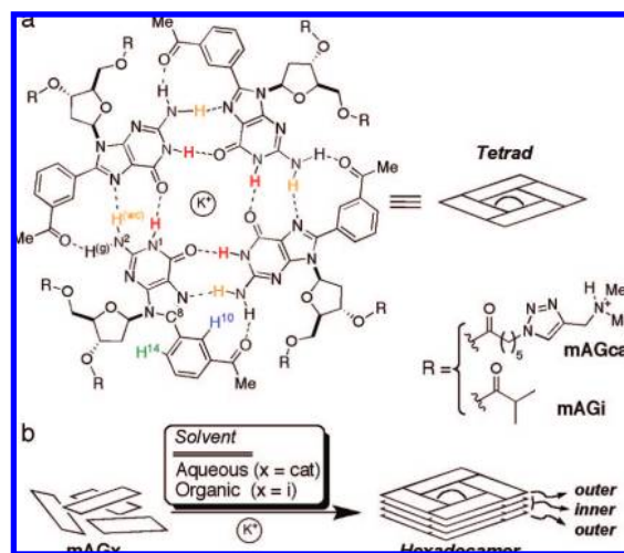
Figure 1. (a) Chemical structure of the mAG tetrad. (b) Cartoon representation for the formation of a hexadecamer formed by mAGx derivatives in aqueous or organic media. A hexadecamer is composed of two sets of tetrads that occur in distinct chemical environments.
